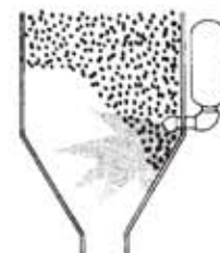
ARCHING at end or above sloping section.
